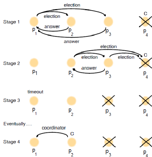
The election of coordinator p_2 , after the failure of p_4 and then p_3
