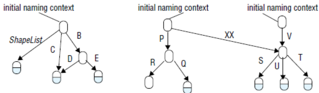
Naming graph in CORBA Naming Service
